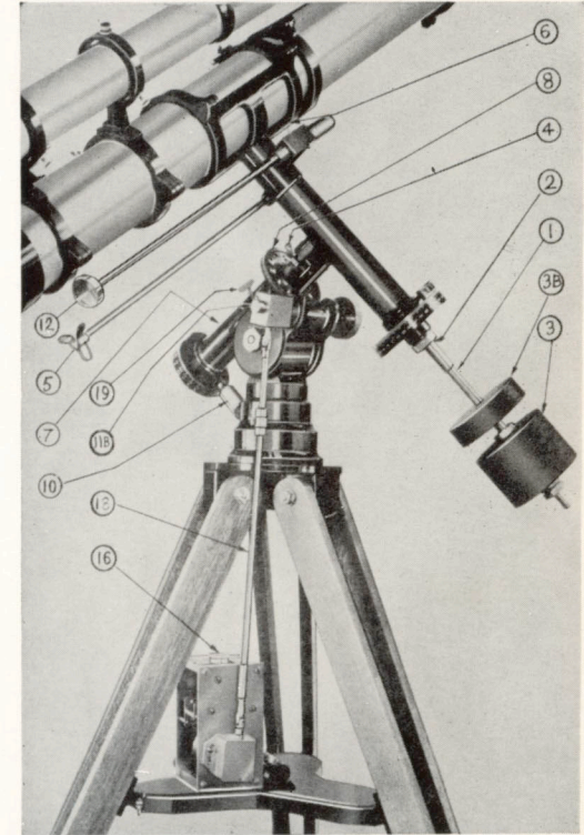
Equatorial Mounting with weight clock drive
